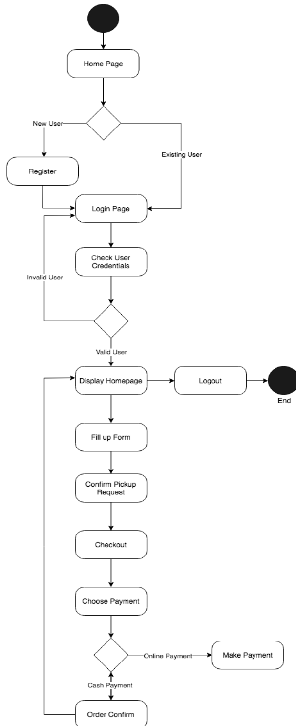
Figure-5.2: Activity Diagram
