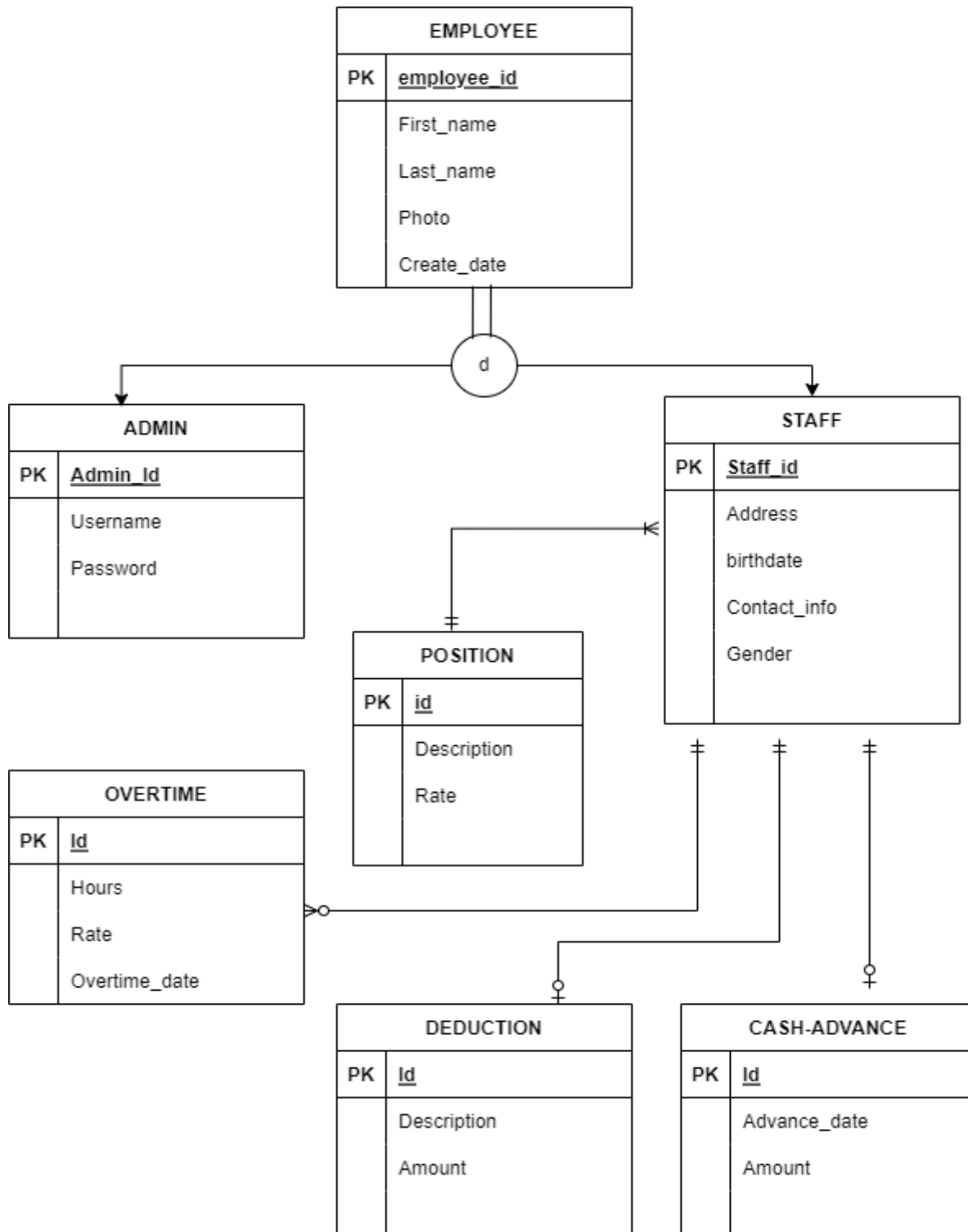
Figure 5.5: ERD for payroll management system
