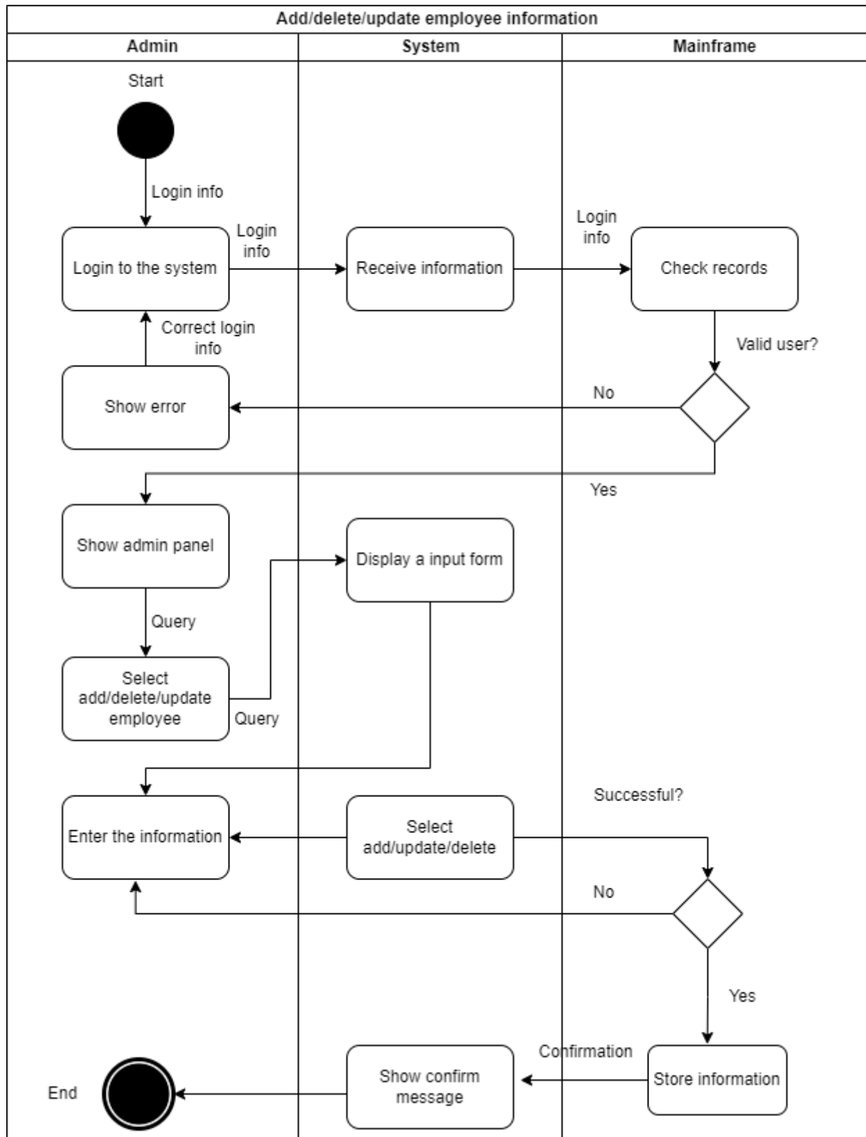
Figure 5.4: Activity diagram
