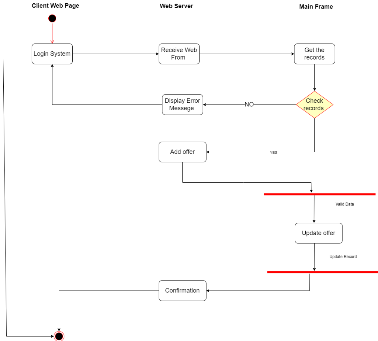
Figure-5.4 Activity Diagram 3
