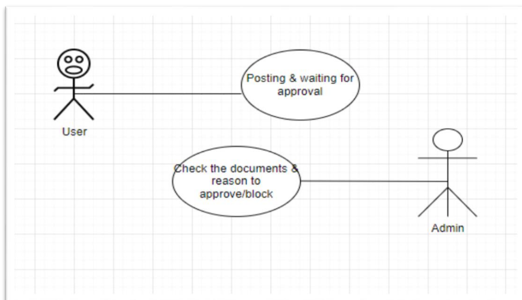
Fig 5.2.3: Post approval
