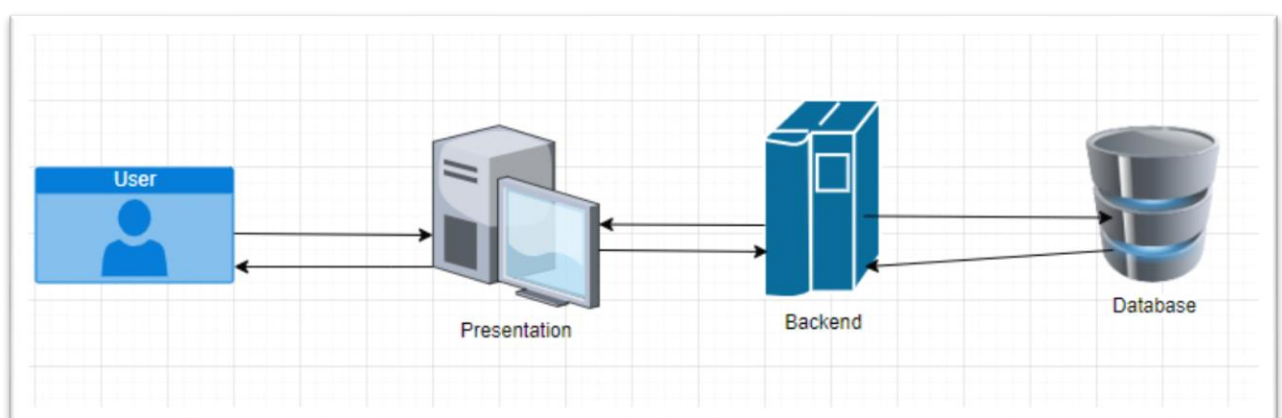
Fig 5.5: Architecture
