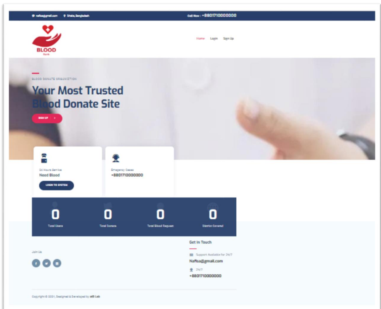
Fig 6.1: Home Page
