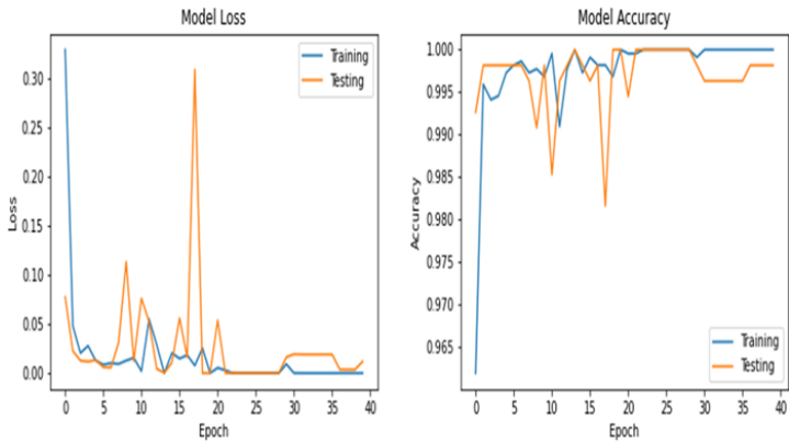
Fig 7: Dense Net model accuracy graph
