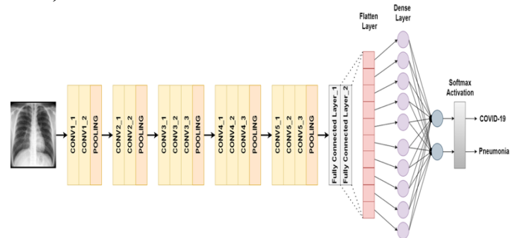
Fig 1: VGG 16 for binary Classification
