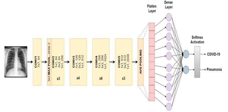
Fig 4: Resnet 50 for binary Classification
