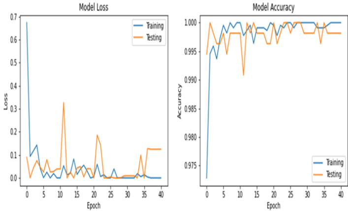
Fig 5: VGG 16 model accuracy graph
