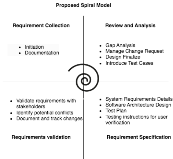
Figure 5: Proposed Model.
