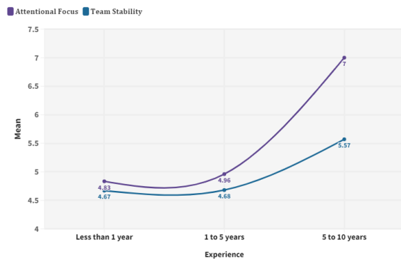
Figure 9: Change of Impact Level of Factors with Respect to Professionals' Experience
