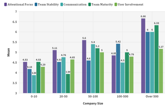
Figure 10: Change of Impact Level of Factors with Respect to Company Size
