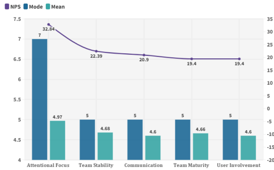
Figure 6: Top Five Factors for On-Time Software Project Delivery During COVID-19
