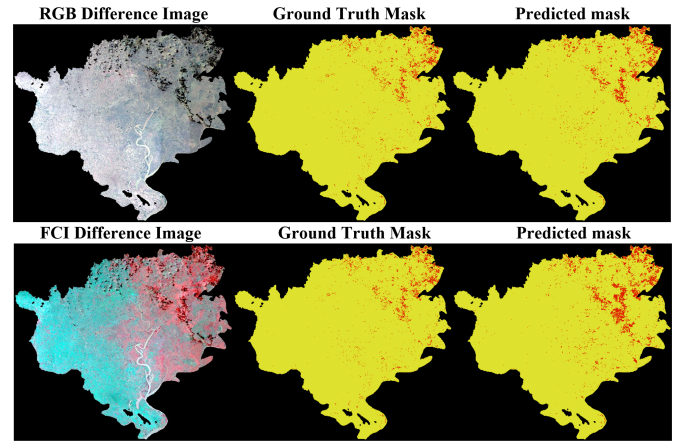
Fig. 24. 2020's RGB and FCI difference images with ground truth mask and predicted mask
