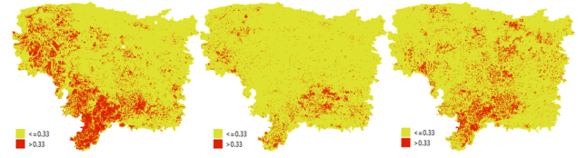
Fig. 5. Sunamganj NDVI different from left to right 2019, 2020 & 2021
