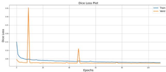
Fig. 19. Training vs Validation dice loss for RGB images
