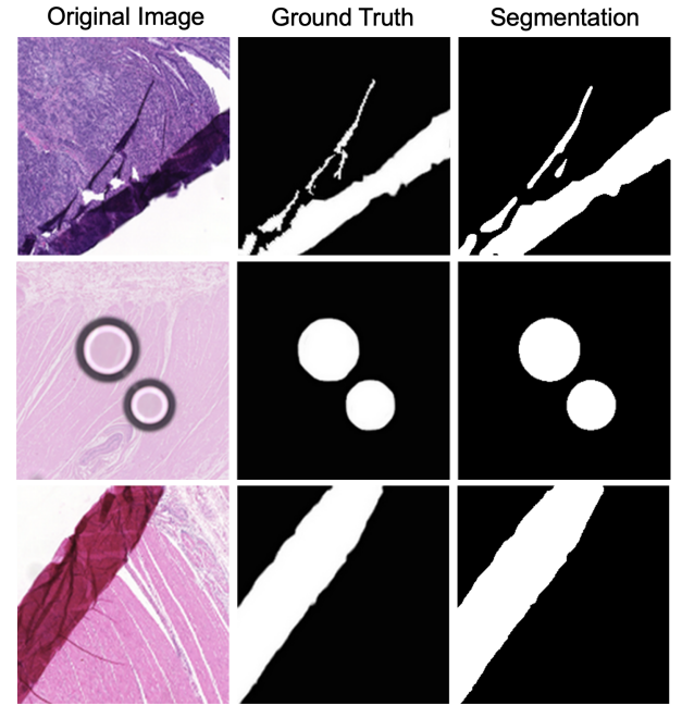
FIGURE 8. Artifact segmentation result by proposed networks.
