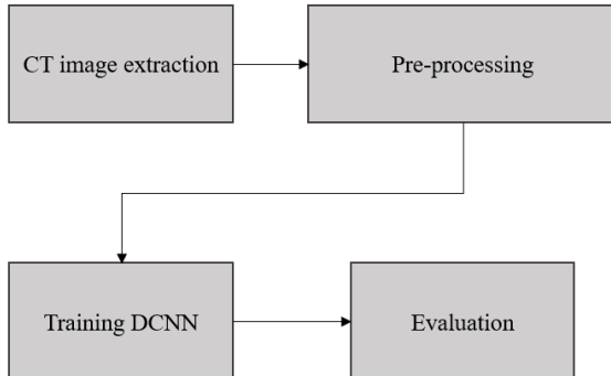
Figure 1: Methodology overview
