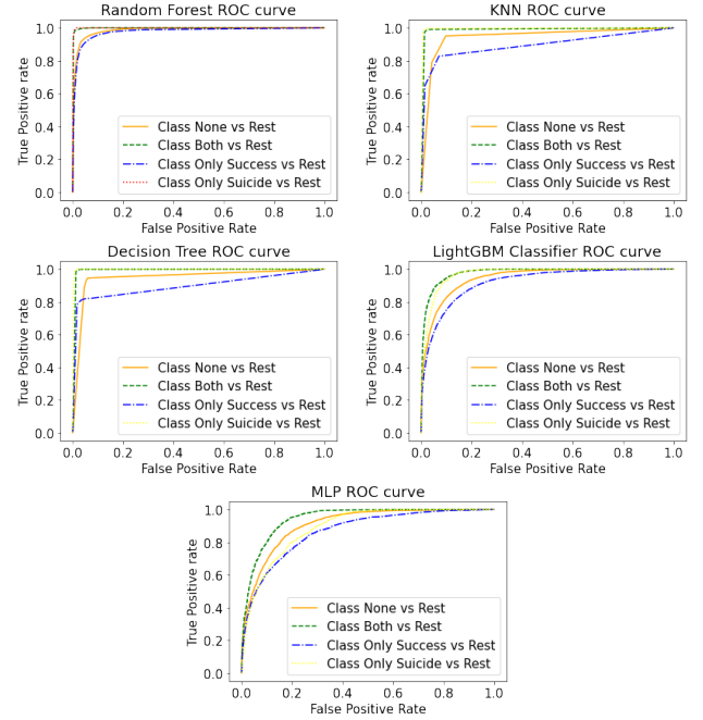
Fig. 7. ROC curves for Different Machine Learning and Artificial Neural Network Algorithms.
