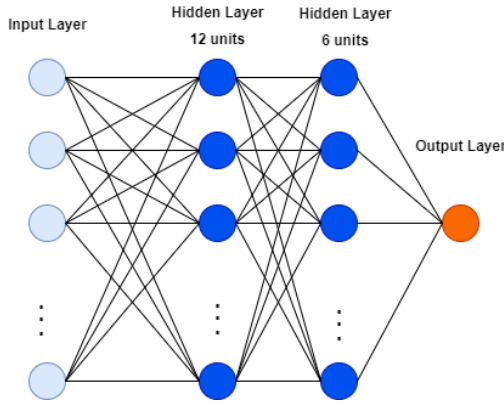
Fig. 4. Architecture of the MLP Model.
