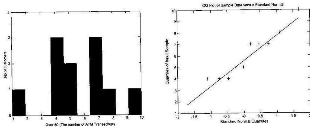
Figure IV - Histogram and QQ plot of over 60
