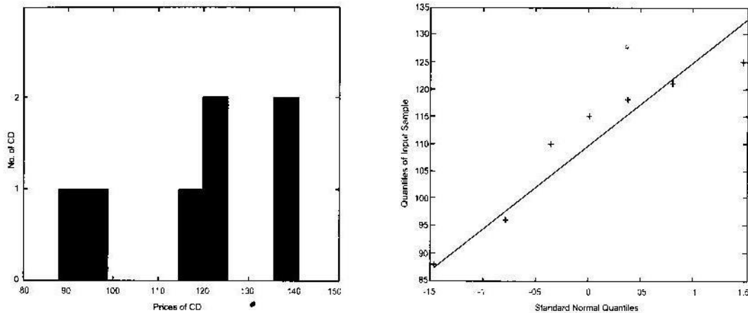
Figure I - Histogram and QQ plot of regular price of compact disc
