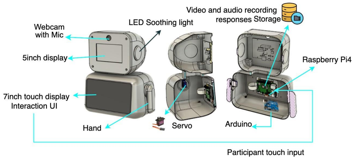
Figure 19: 3D Model Block Diagram
