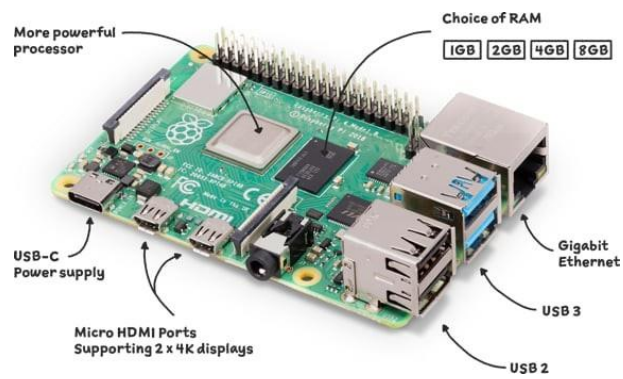
Figure 40: Raspberry Pi 4B [71]
