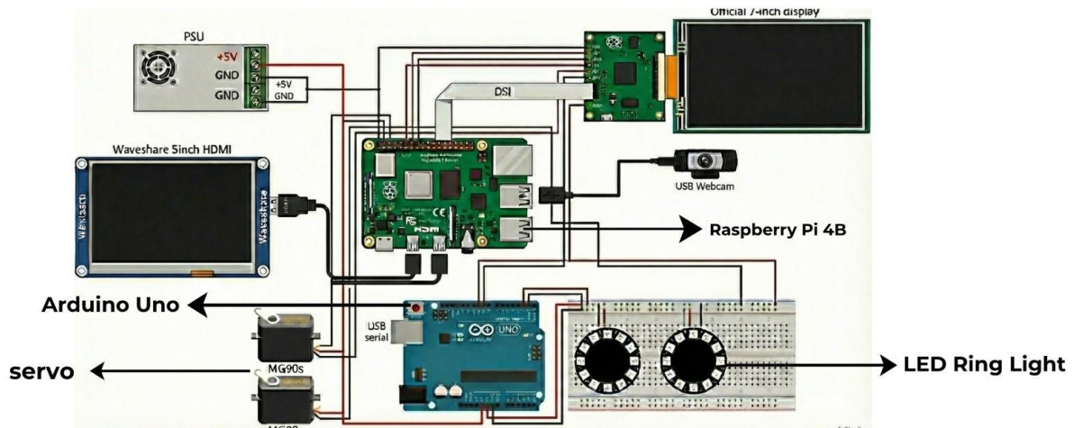
Figure 39: Hardware Architecture
