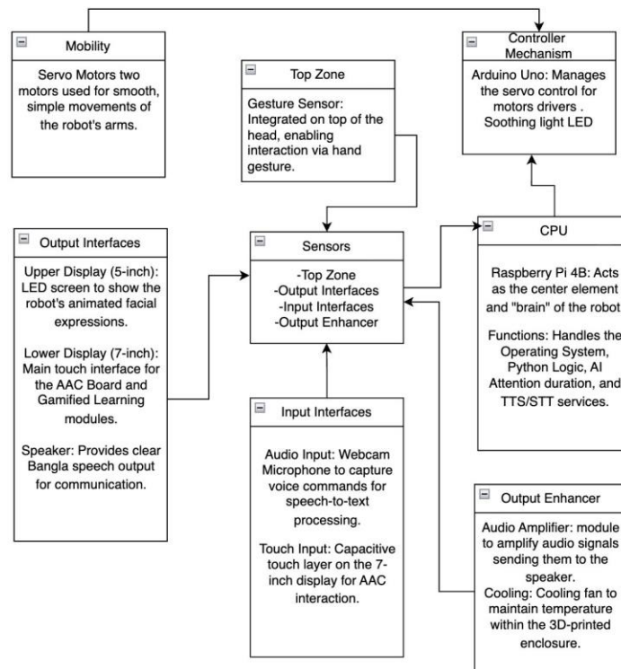
Figure 18: Hardware Block diagram
