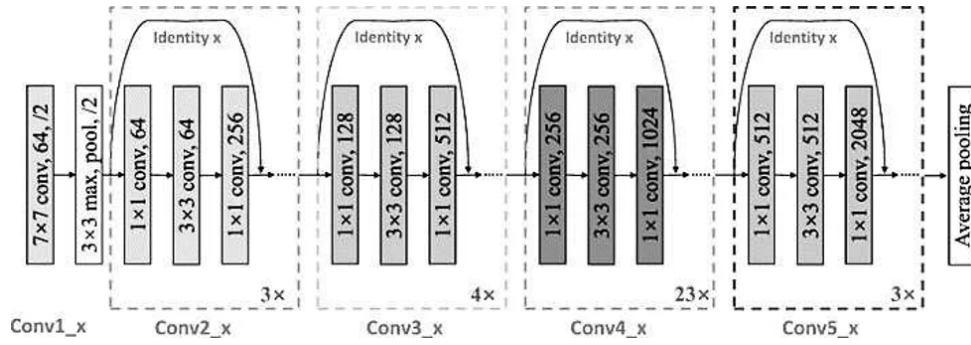
Figure 4.7: ResNet-101 layer configuration [38].
