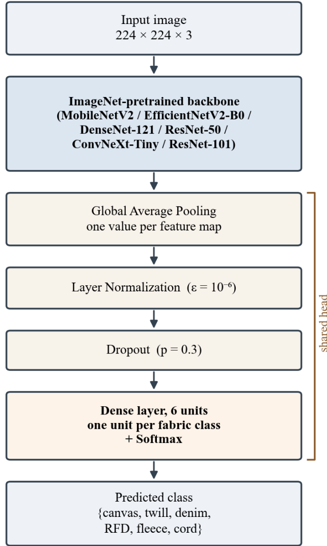
Figure 4.8: Model architecture used across all six experiments.
