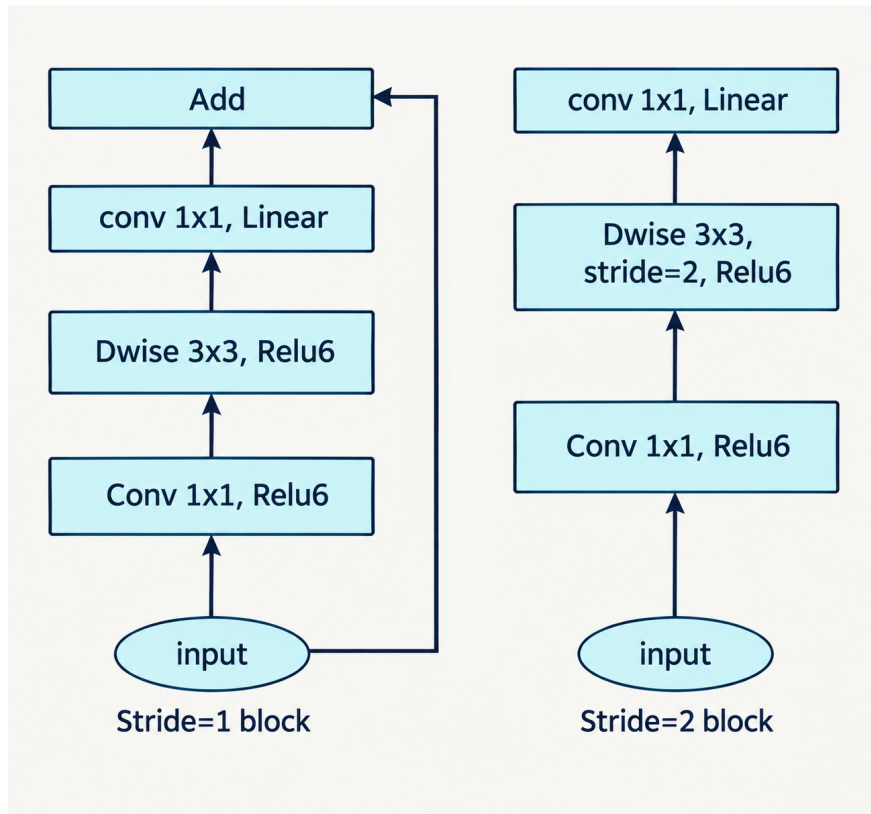
Figure 4.2: MobileNetV2 inverted residual blocks [13].
