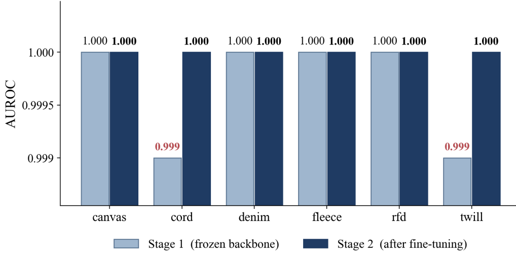
Figure 5.4: Per-class AUROC before and after fine-tuning.
