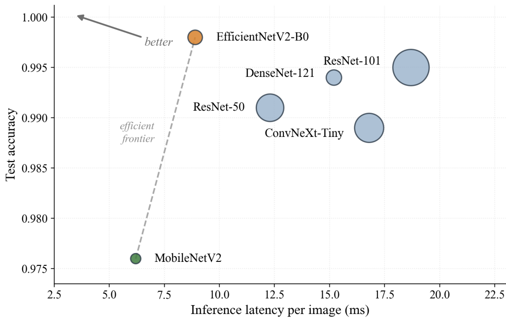
Figure 5.7: Test accuracy against inference latency.
