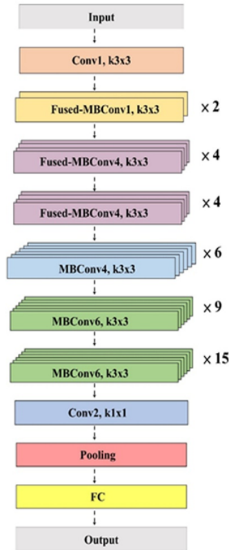
Figure 4.3: EfficientNetV2-B0 stage layout [14].
