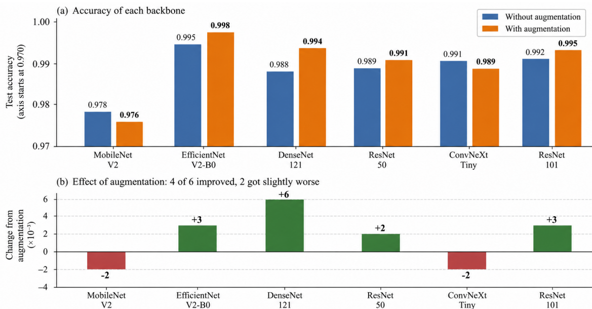
Figure 5.1: Test accuracy and the effect of augmentation.
