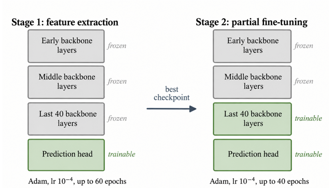
Figure 4.9: Two-stage transfer-learning schedule.
