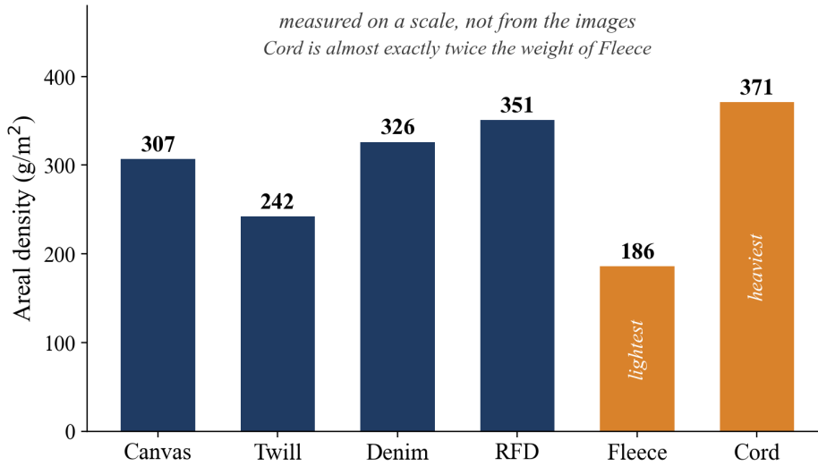
Figure 3.2: Measured areal density per class.
