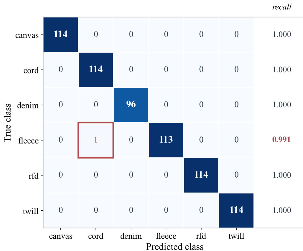
Figure 5.3: Confusion matrix on the held-out test partition.
