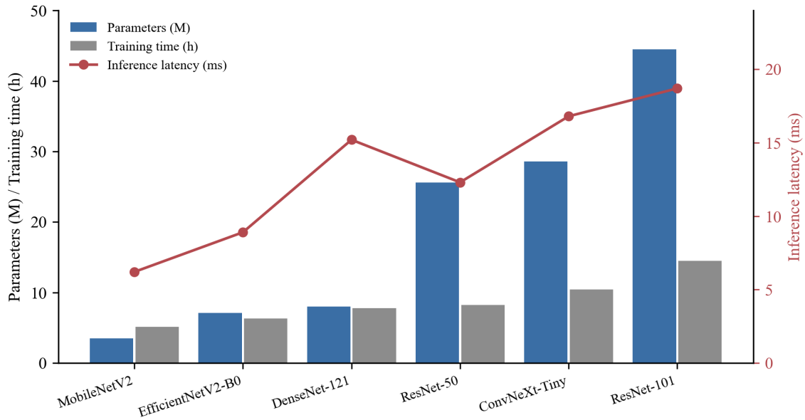
Figure 5.6: Parameter count, training time and inference latency.
