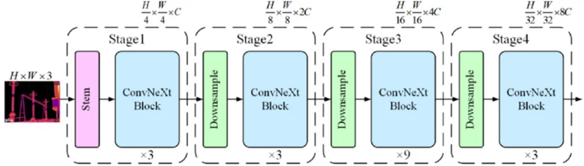
Figure 4.6: ConvNeXt four-stage layout [37].
