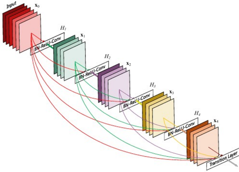
Figure 4.4: Dense connectivity within a DenseNet block [15].
