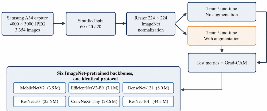
Figure 4.1: Experimental pipeline from capture to backbone comparison.
