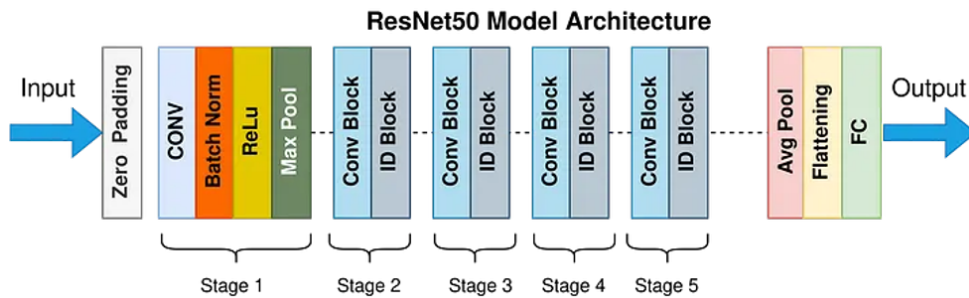
Figure 4.5: ResNet-50 stage architecture [36].
