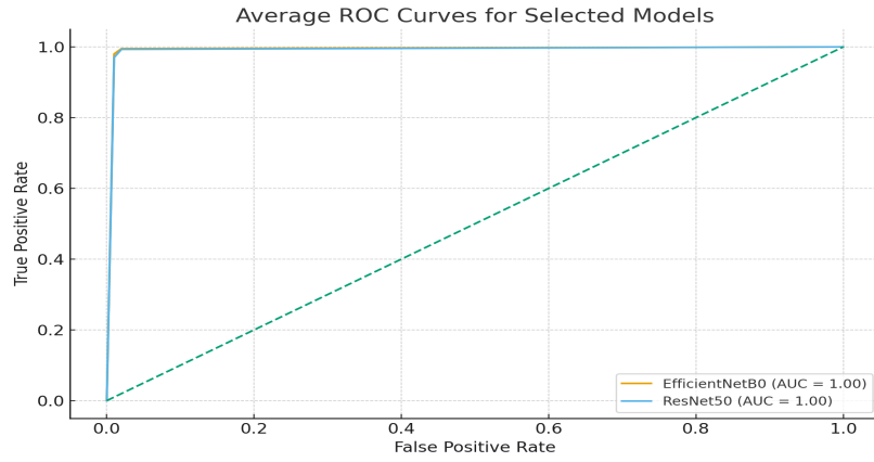
Figure 5.3: Average macro AUROC for all models across BdSL, ASL and ISL
