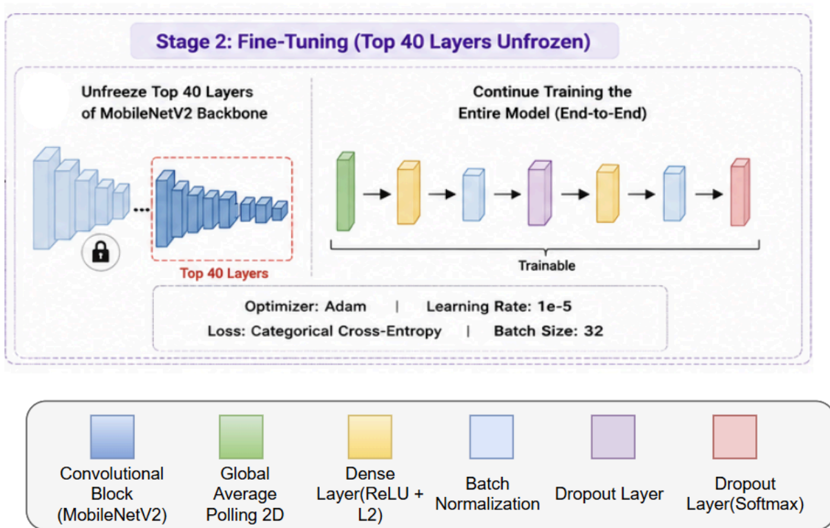
Figure 4.8 : Phase 2 focused on fine-tuning the pretrained MobileNetV2 model.
