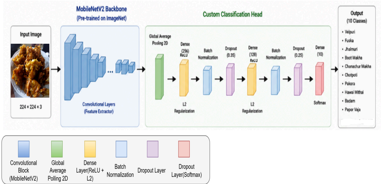
Figure 4.6: Proposed MobileNetV2 Custom head classification.
