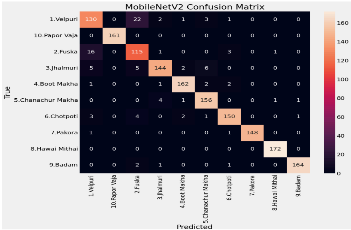
Figure 6.6: Confusion Matrix of MobileNetV2 on the Test Dataset .
