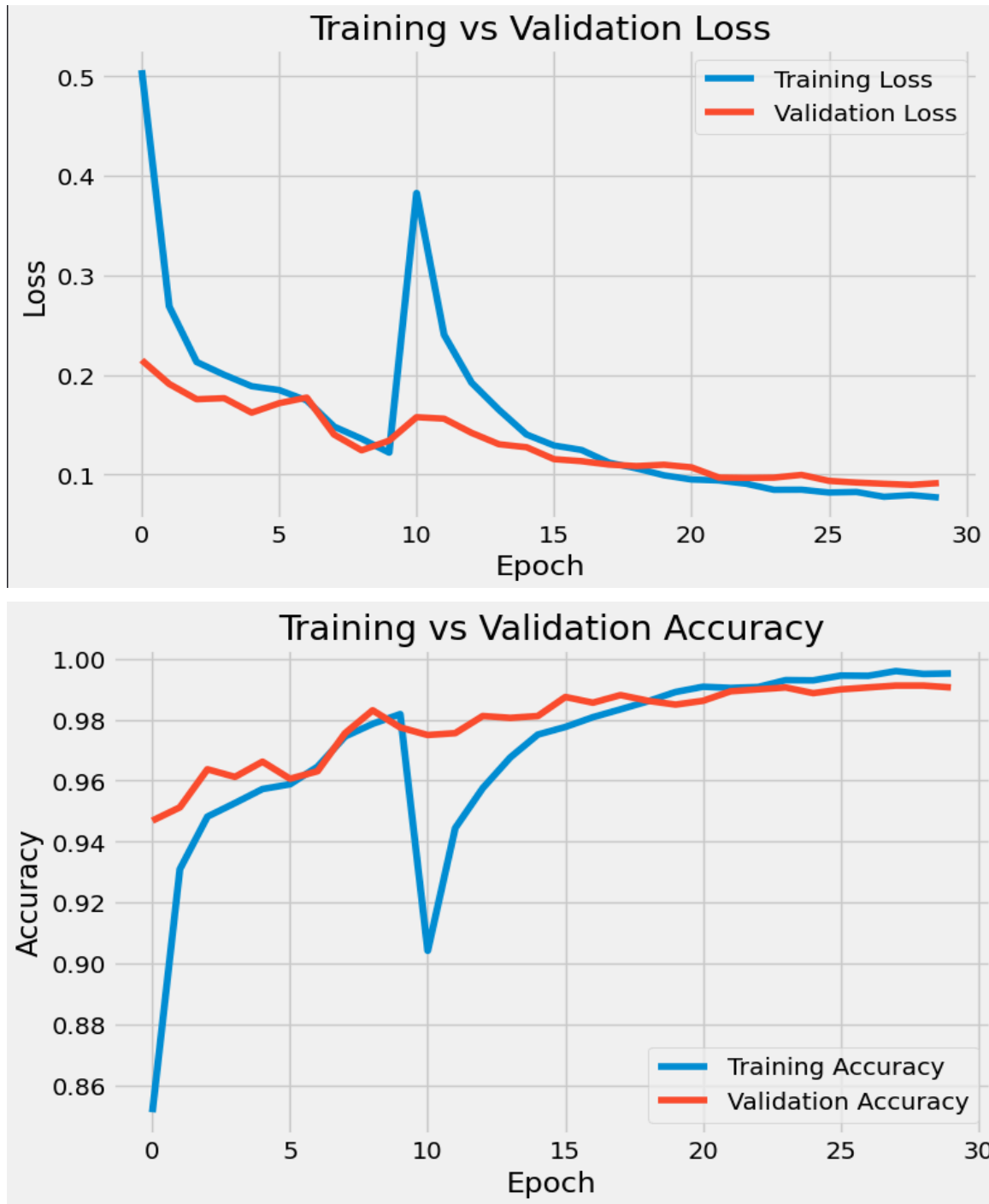
Figure 6.11: Training and Validation Loss and Accuracy Curves of the Proposed Two-Stage MobileNetV2 Model .
