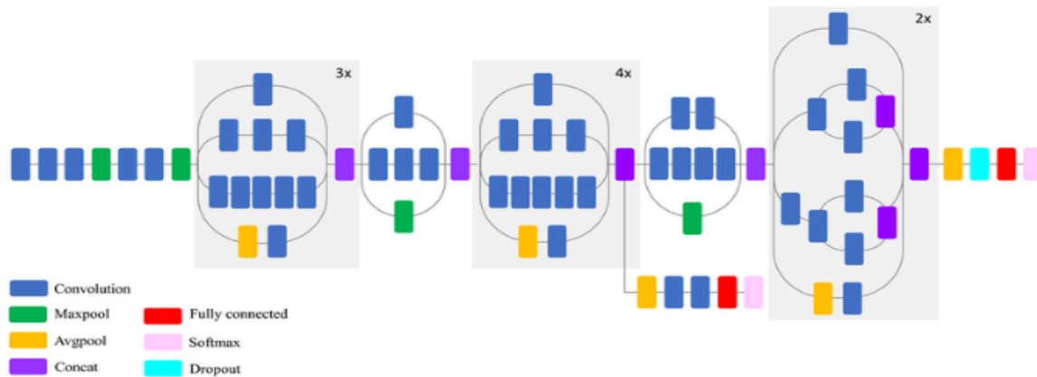
Figure 4.9: Architecture of the InceptionV3 transfer learning model used in this study.
