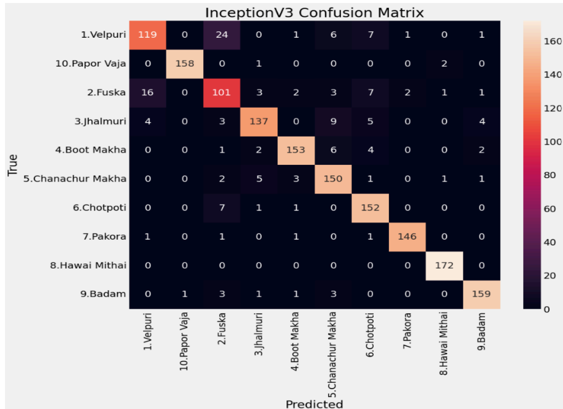
Figure 6.2: Confusion Matrix of InceptionV3 on the Test Dataset .
