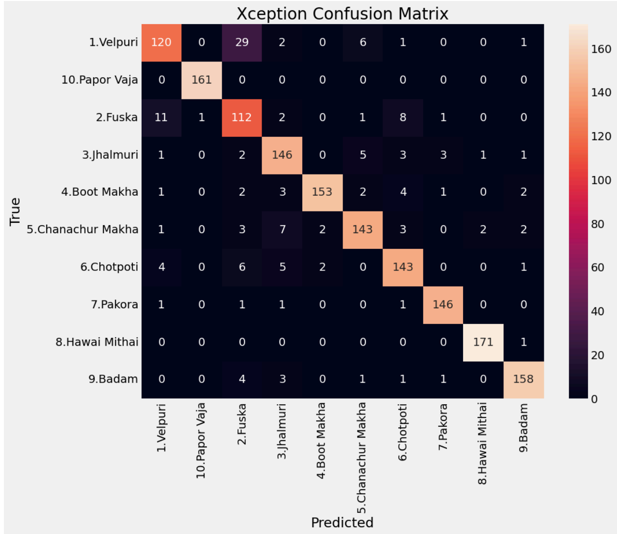
Figure 6.10: Confusion Matrix of Xception on the Test Dataset.
