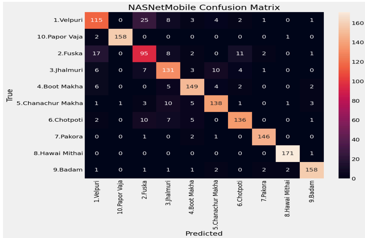
Figure 6.7: Confusion Matrix of NASNetMobile on the Test Dataset
