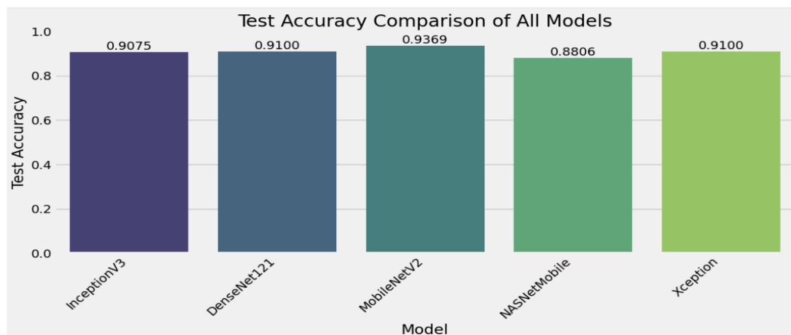
Figure 6.13: Comparative Test Accuracy of the Evaluated Transfer Learning Models .
