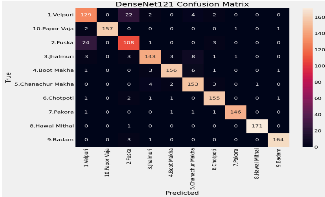
Figure 6.4: Confusion Matrix of DenseNet121 on the Test Dataset .
