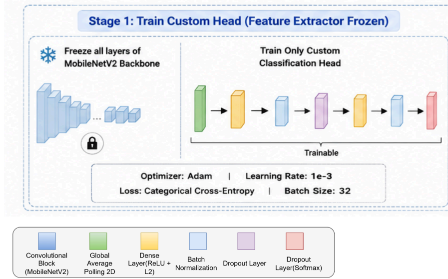
Figure 4.7: Phase 1 of proposed MobileNetV2 Architecture with Custom Classification Head.
