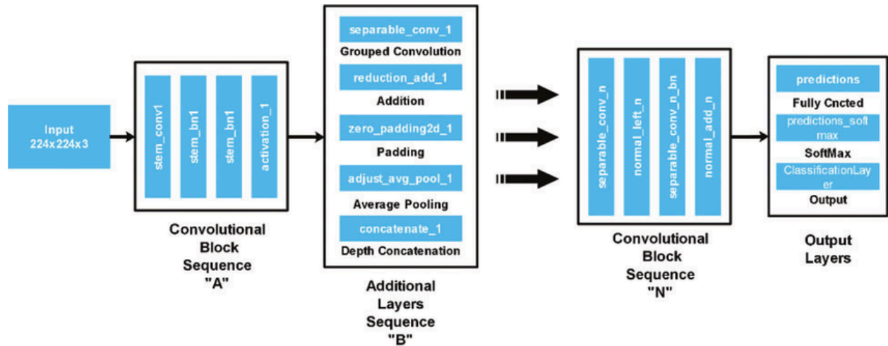
Figure 4.12: NASNetMobile transfer learning architecture.
