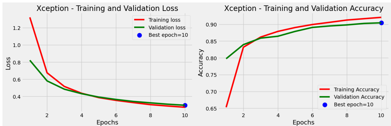
Figure 6.9: Training and Validation Loss and Accuracy Curves of Xception.
