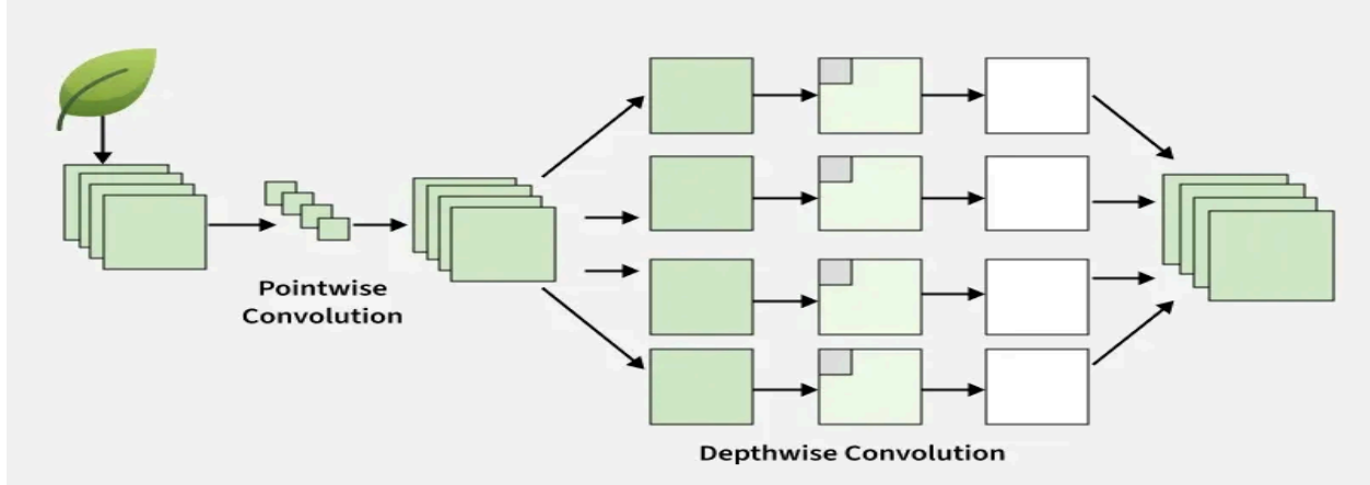
Figure 4.13: Xception transfer learning architecture.
