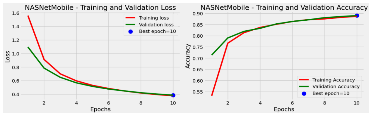
Figure 6.8: Training and Validation Loss and Accuracy Curves of MobileNetV2.
