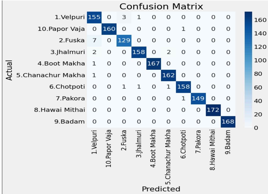
Figure 6.12: Confusion Matrix of the Proposed Two-Stage MobileNetV2 model on the Test Dataset .
