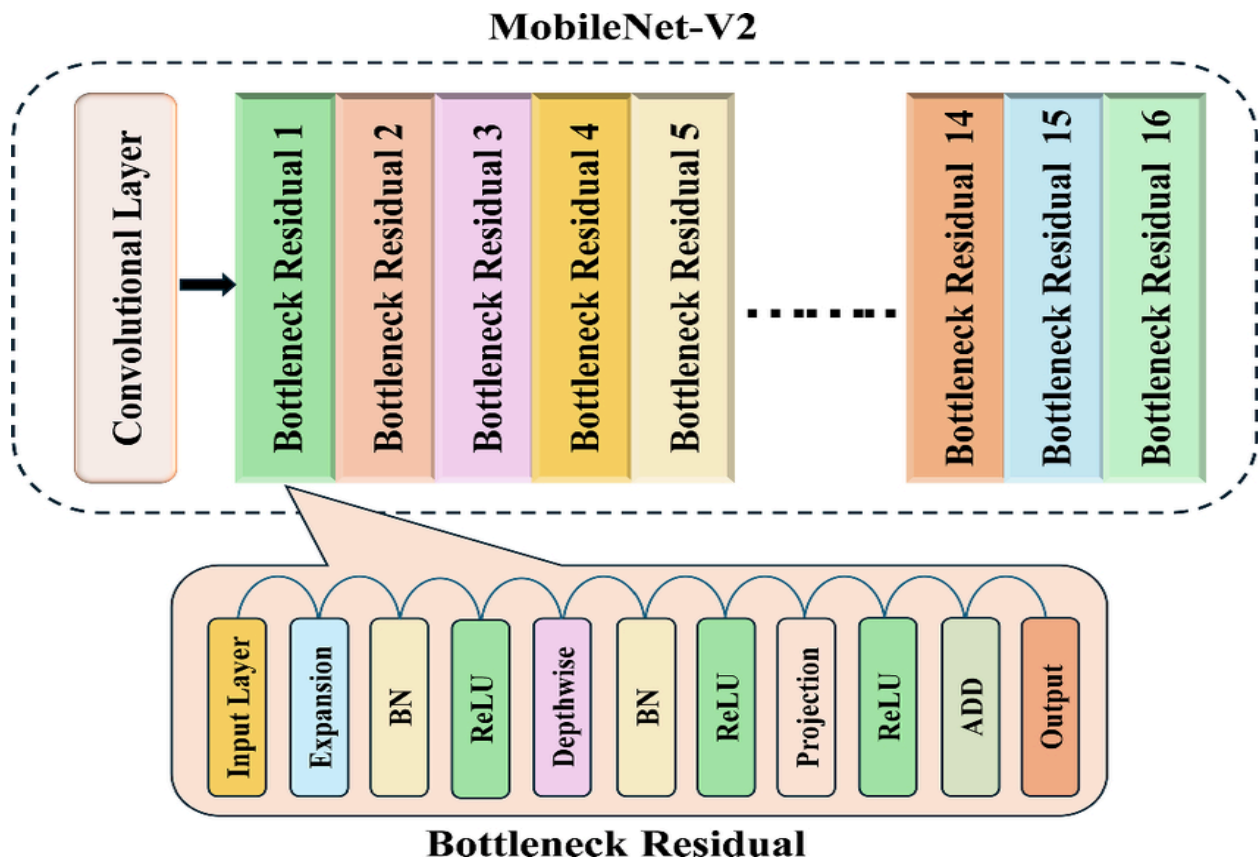
Figure 4.10: Baseline MobileNetV2 transfer learning architecture.
