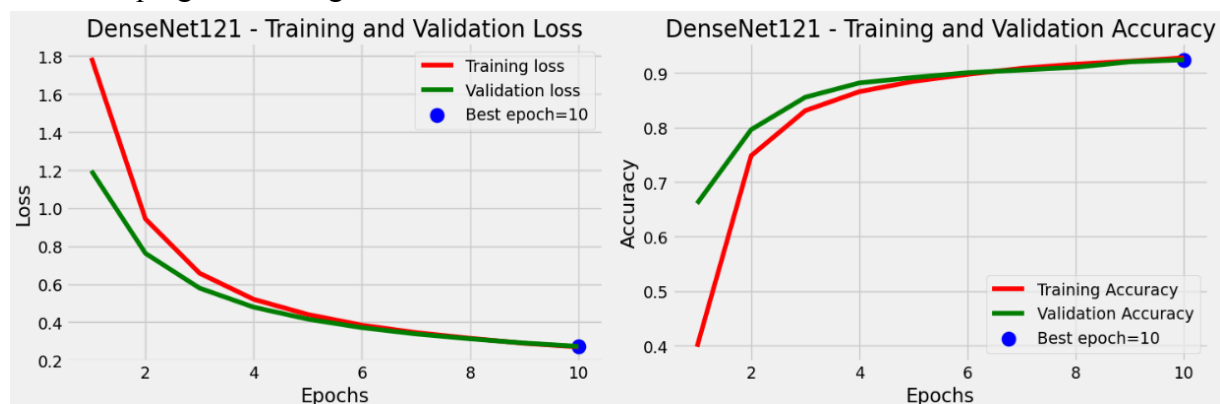
Figure 6.3: Training and Validation Loss and Accuracy Curves of DenseNet121.
