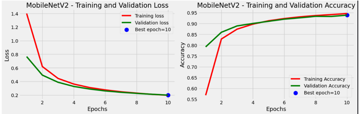
Figure 6.5: Training and Validation Loss and Accuracy Curves of MobileNetV2.
