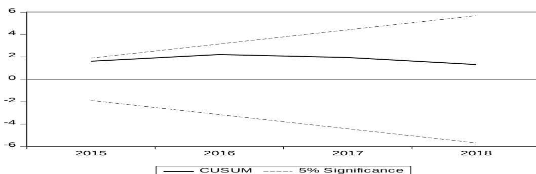
Figure A: CUSUM test for ARDL Model Stability
