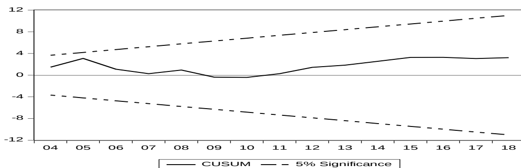
Figure C: CUSUM test for Long Run Model Stability
