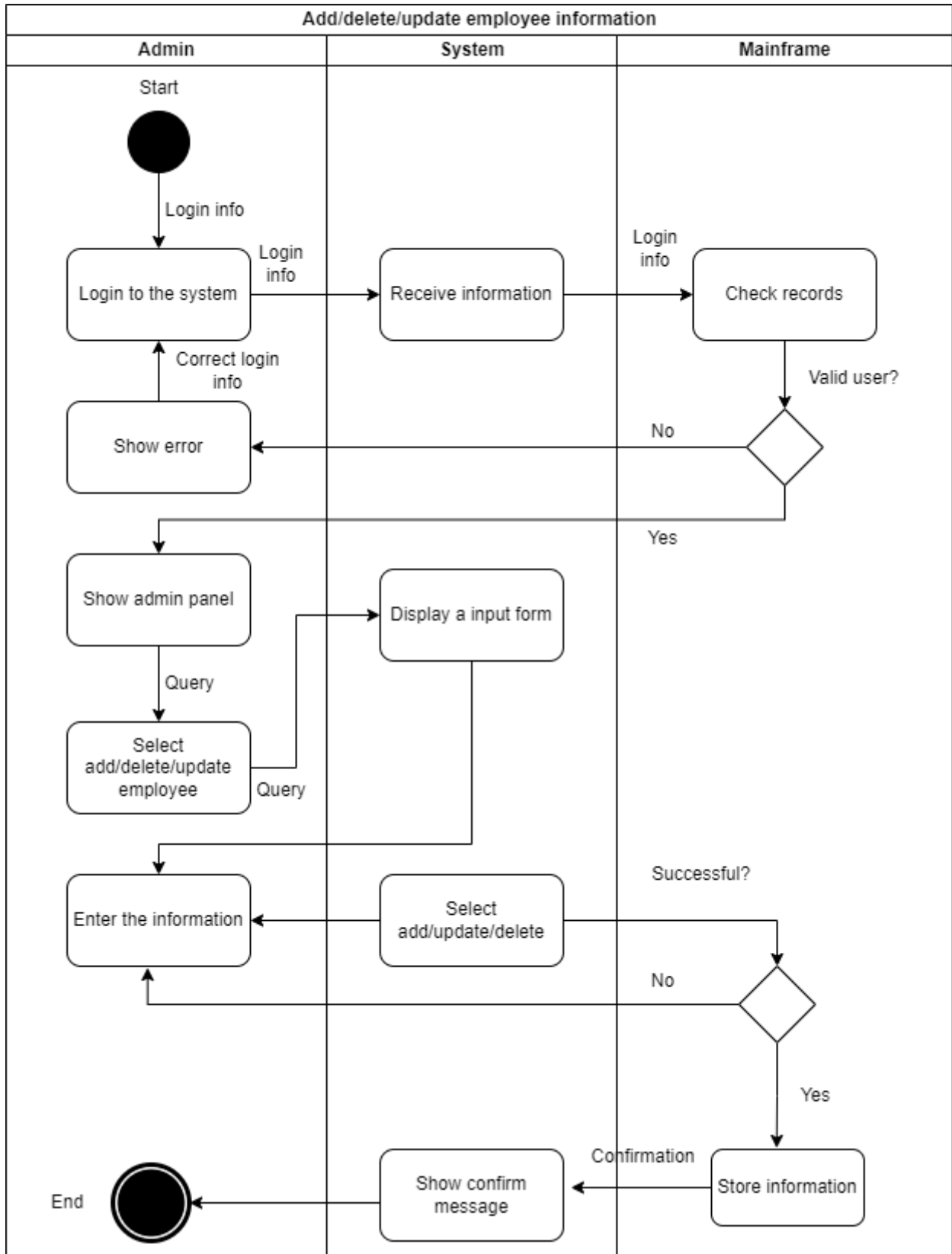
Figure 5.4: Activity diagram
