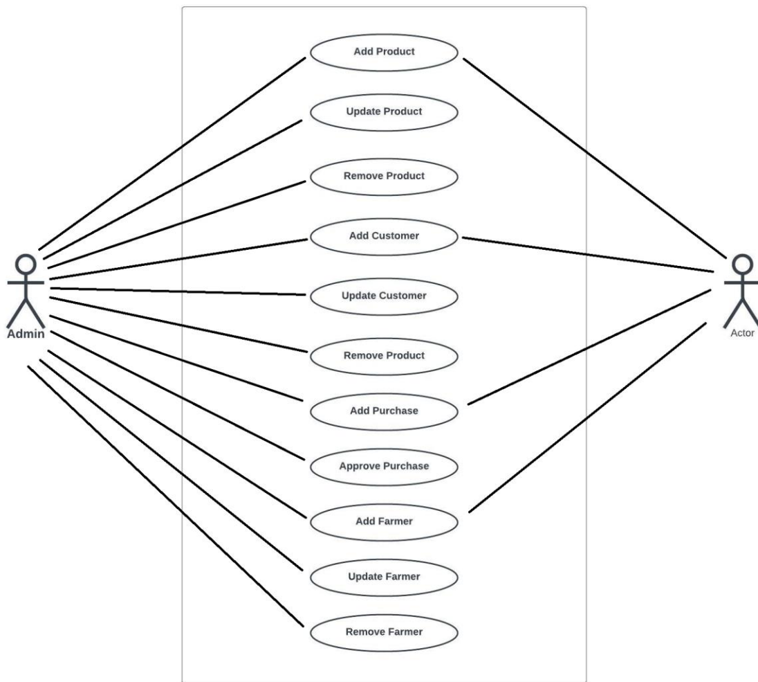
Figure 5.2: Use Diagram
