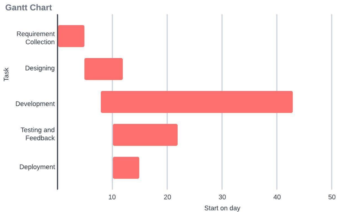
Figure 3.2: Gantt Chart
